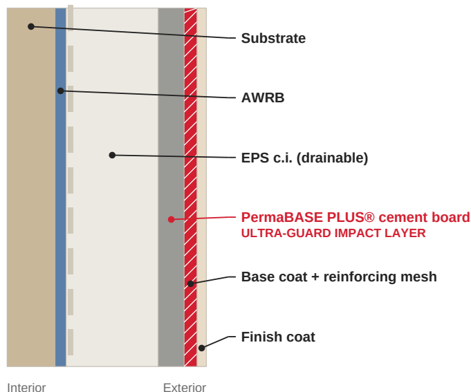
TYPICAL ULTRA-GUARD WALL SECTION
